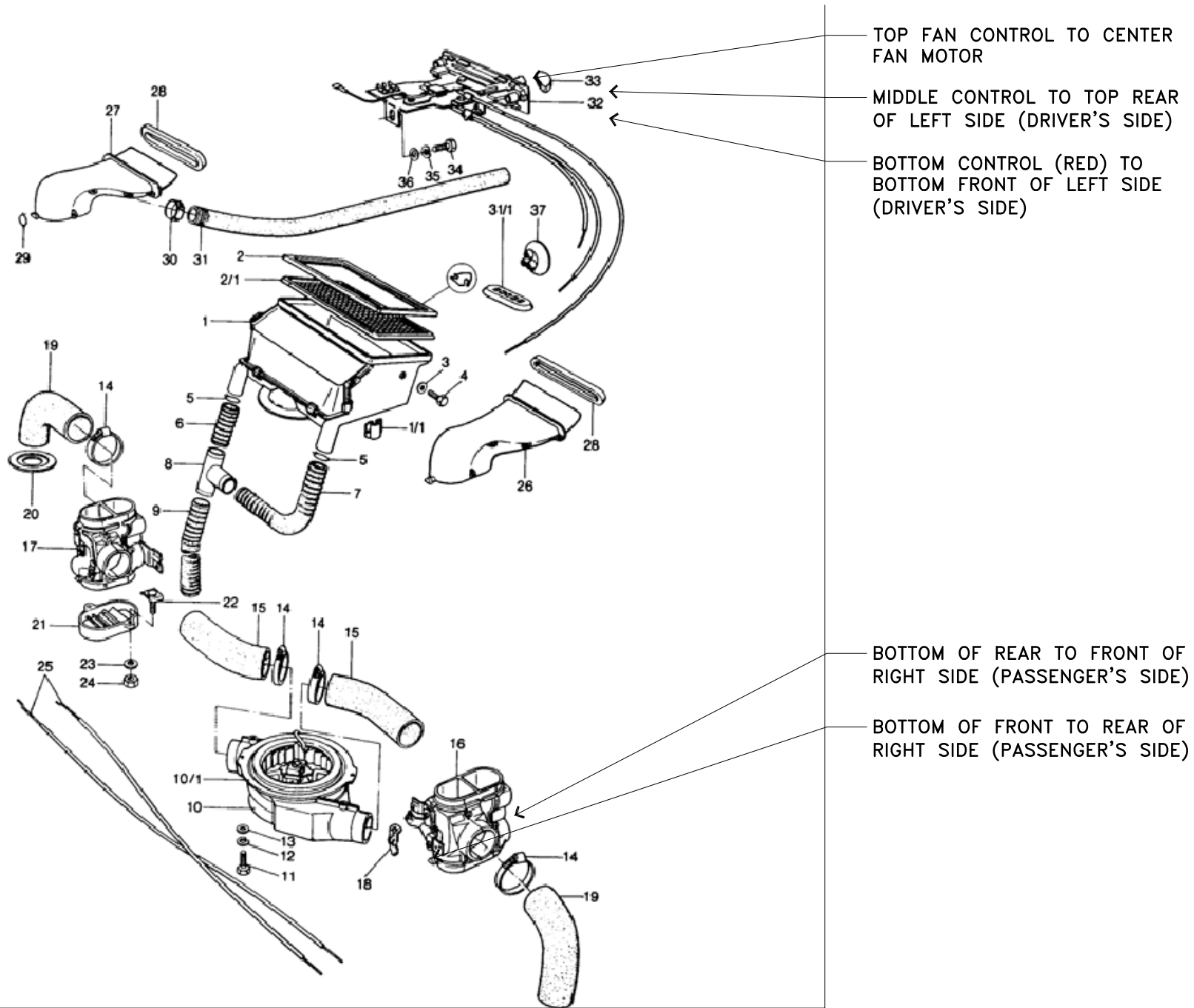
HEATER/VENTILATION CABLE ROUTE
